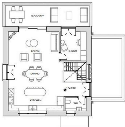
PROPOSED FIRST FLOOR PLAN 1:100
